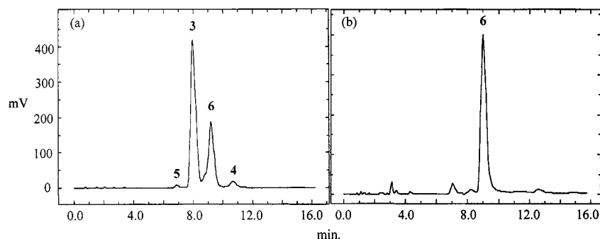
Figure 1. HPLC (eluent \text{CH}_3\text{CN}:\text{H}_2\text{O} , 80%:20%, detection UV, \lambda = 254 \text{ nm} ) trace of the 1200^\circ\text{C} pyrolysate of 3 before (a) and after (b) isolation of 6
