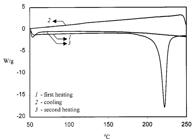
Figure 3. DSC trace of 15 (first and second heating run as well as first cooling run, see Experimental Section; -W/g exothermic)
