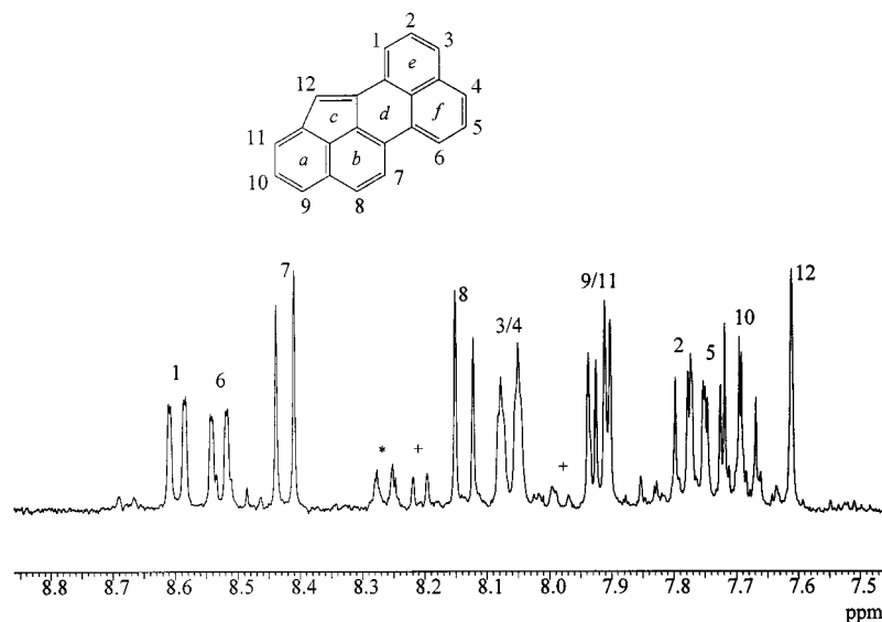
Figure 2. ^1\text{H} NMR (300.13 MHz, [\text{D}_6]\text{acetone} ) of 6 isolated by preparative HPLC; * and + traces of cyclopenta[ cd ]perylene ( 5 ) and perylene ( 13 )
